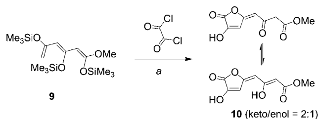
Scheme 2. Synthesis of \gamma -(2,4-dioxobut-1-ylidene)butenolide 10 . a ) Oxalyl chloride, Me 3 SiOTf (0.3 equiv.), CH 2 Cl 2 , –78 → 20 °C, 12 h, 55%.
