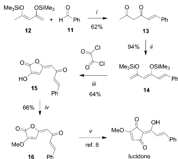
Scheme 3. Formal synthesis of lucidone: i ) TiCl 4 (1.0 equiv.), CH 2 Cl 2 , –78 → 20 °C. ii ) Me 3 SiOTf (2.0 equiv.), NEt 3 , Et 2 O, 0 → 20 °C. iii ) Oxalyl chloride, Me 3 SiOTf (0.5 equiv.), CH 2 Cl 2 , –78 → 20 °C. iv ) Me 2 SO 4 , K 2 CO 3 , acetone, 20 °C. v ) NaOMe, MeOH (ref. [8] ).
