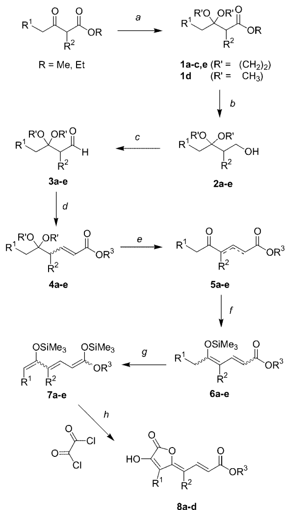
Scheme 1. Synthesis of 1,5-bis(trimethylsilyloxy)-1,3,5-hexatrienes 7a–e and butenolides 8a–d . a ) 1a–c,e : (CH 2 OH) 2 , p TsOH, toluene, Dean–Stark trap, reflux, 12 h, 77–80%; 1d : (MeO) 3 CH, Amberlist IR-120 + , 20 °C, 62%. b ) (iBu) 2 AlH, CH 2 Cl 2 , –78 → 20 °C, 2 h, 20%, 1 h, 60–92%. c ) Oxalyl chloride, DMSO, NEt 3 , –78 → 20 °C, 78–95%. d ) Ph 3 P=CHCO 2 R 3 , THF, 20 °C, 1 h, 42–72%. e ) 5a–c,e : p TsOH, acetone, reflux, 12 h, 65–84%; 5d : TFA, CH 2 Cl 2 , 95%. f ) Me 3 SiCl, NEt 3 , C 6 H 6 , 20 °C, 24 h, 77–98%. g ) 1) 1.5 equiv. LDA, HMPA, THF, –78 °C, 1 h, 2) Me 3 SiCl, –78 → 20 °C, 4 h, 70–93%. h ) Oxalyl chloride, 0.5 equiv. Me 3 SiOTf, CH 2 Cl 2 , –78 → 20 °C.
